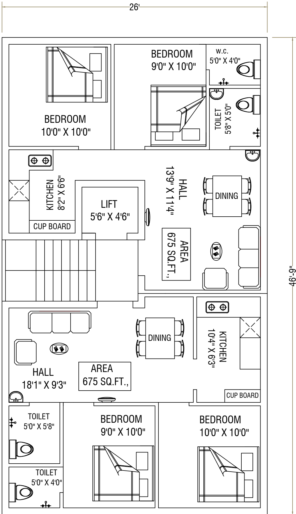
VARADHAPPAN STREET, WEST MAMBALAM FIRST FLOOR PLAN
